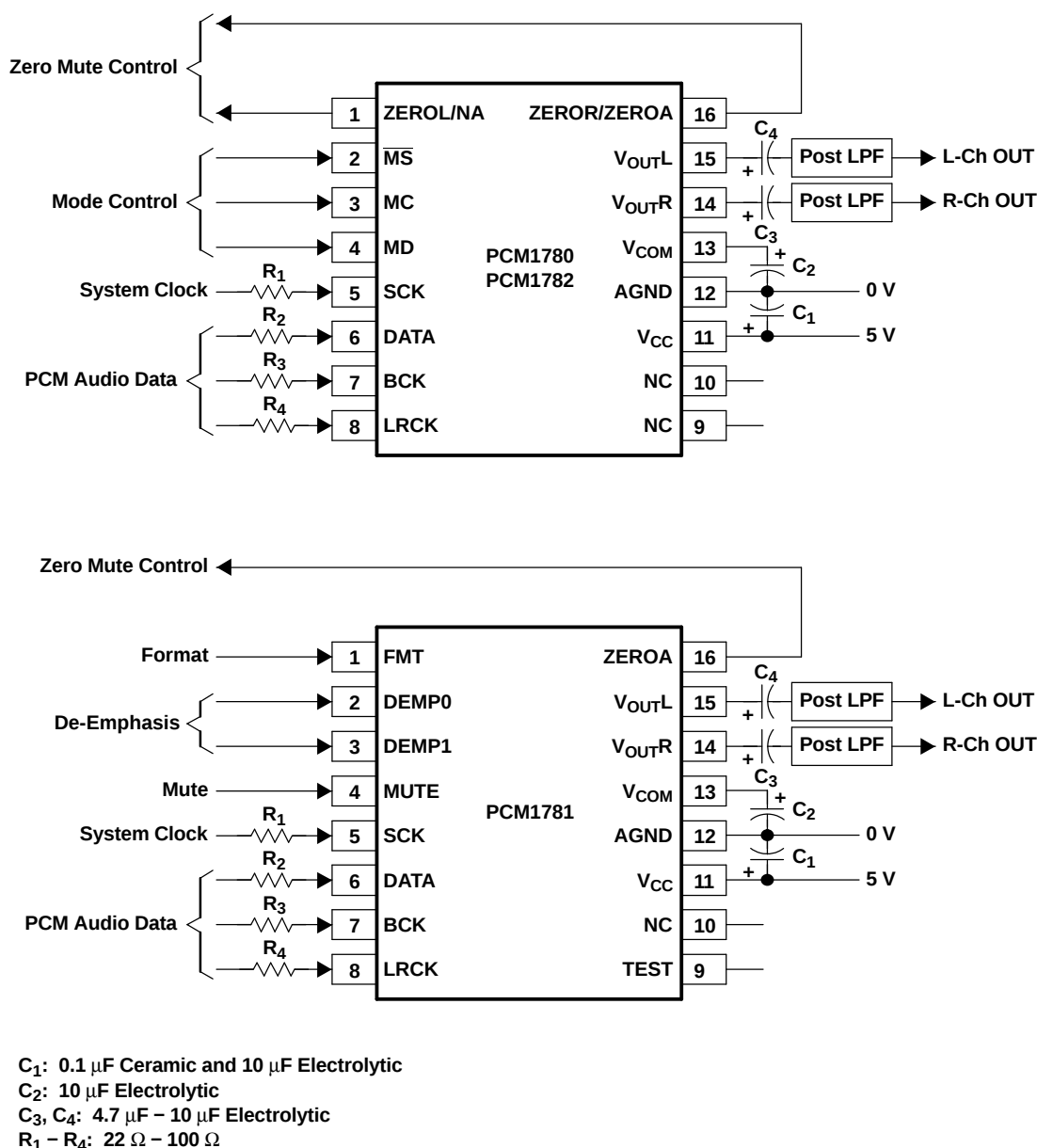
Figure 28. Basic Connection Diagram
