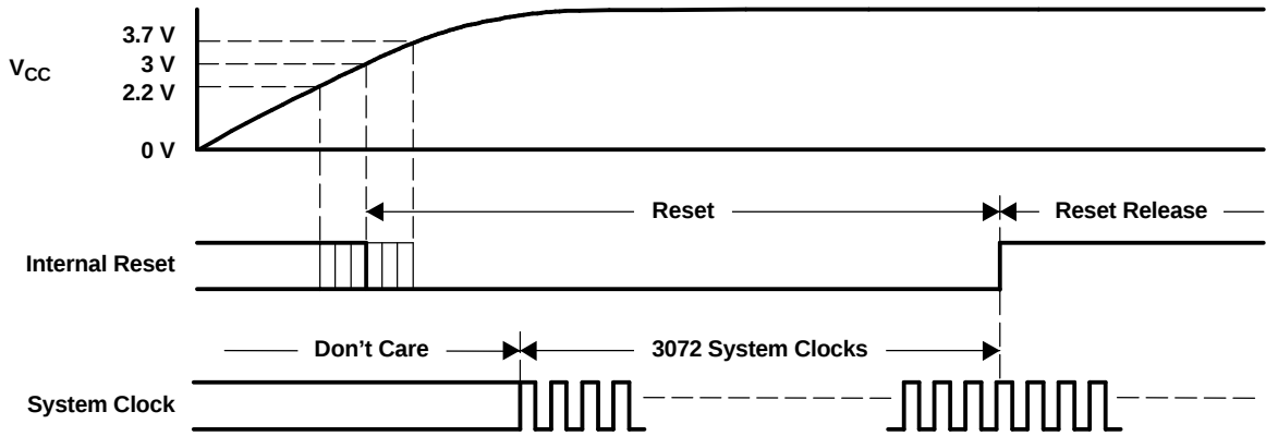
Figure 21. Power-On-Reset Timing
